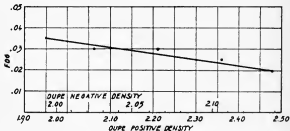
FIG. 9. Fog in final print as a function of combinations of dupe positive and dupe negative densities.
